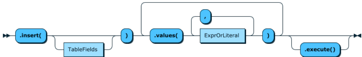
Figure 6.1 Table.insert() Syntax Diagram
