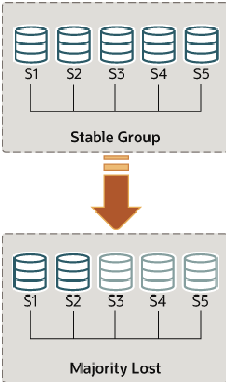
Figure 17.7 Losing Quorum
