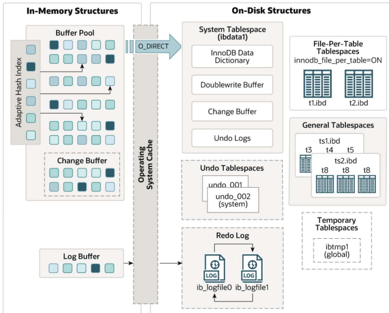
Figure 14.1 InnoDB Architecture
