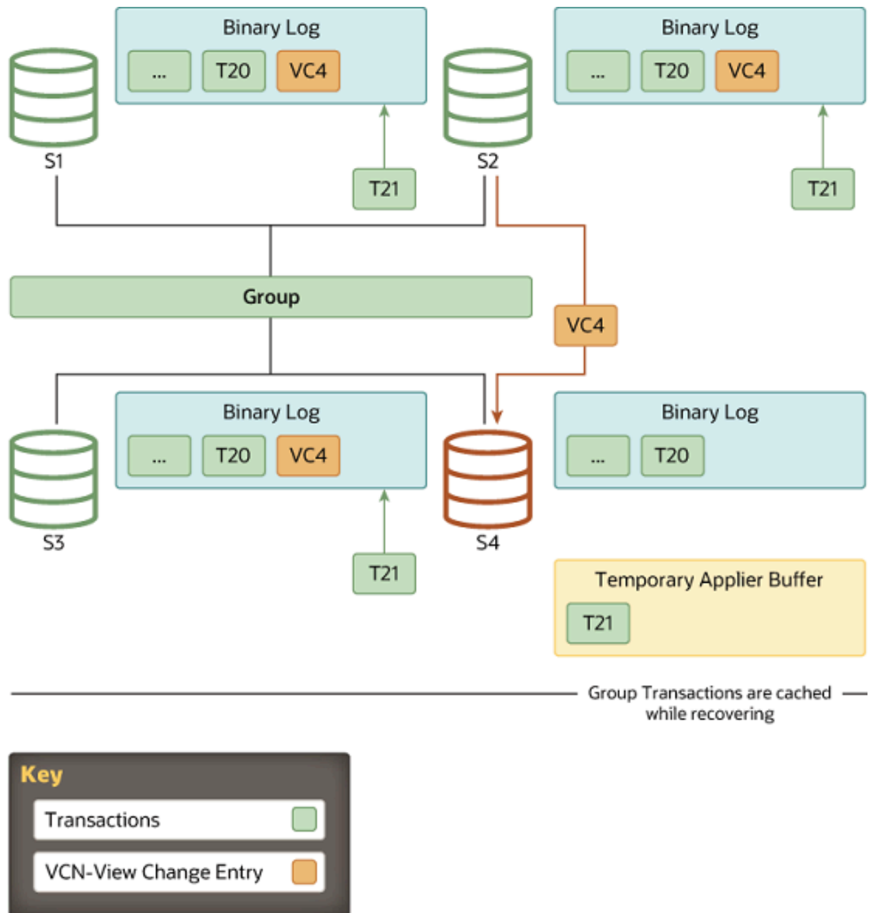
Figure 17.13 Queued Transactions
