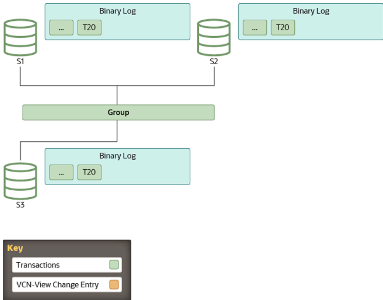
Figure 17.10 Stable Group
