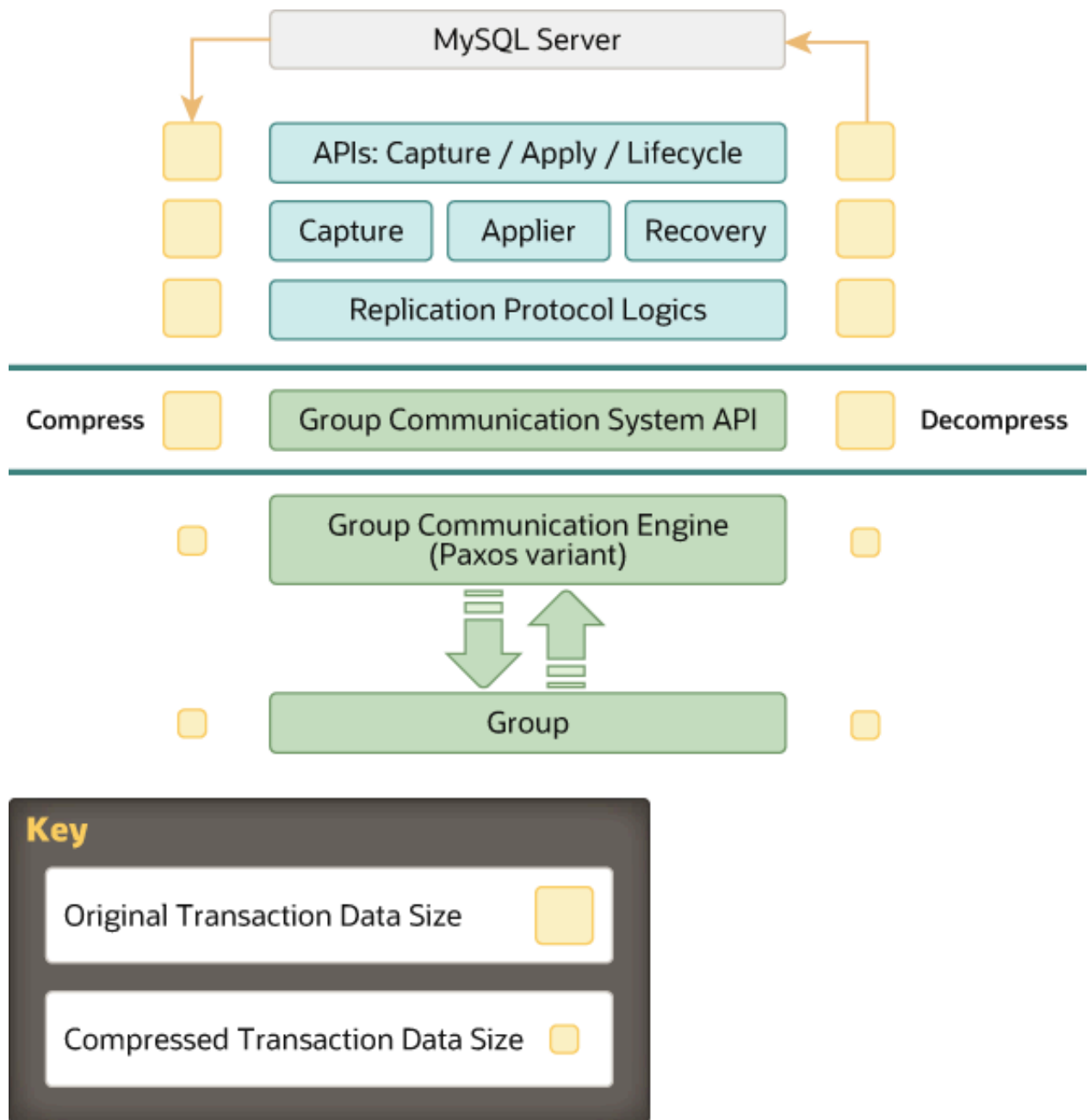
Figure 17.15 Compression Support
