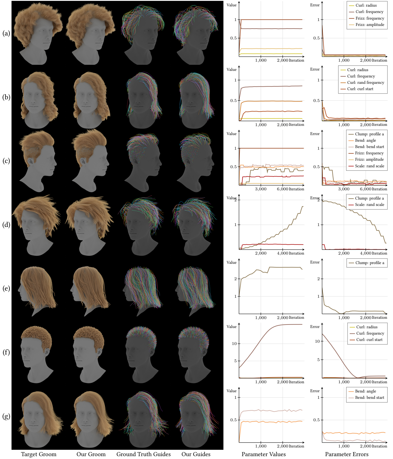
Fig. 7. SYNTHETIC GROOMS. We recover the guide strands and operator parameters of 7 synthetic grooms. We visualize the recovered procedural groom, guide strands, and show parameter values and errors over optimization iterations. Grooms adapted from Hair Styles ©Daniel Bystedt.
