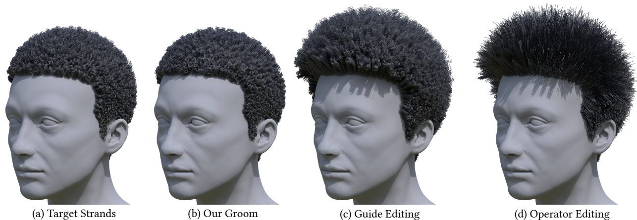
Fig. 1. We design a procedural pipeline that generates hair grooms using a small set of guide strands and artist-friendly hair grooming operators. (a) Given unstructured hair strand geometry, we propose optimization strategies to (b) fit the guide strands and grooming operator parameters of the procedural groom. We can then edit the hair shape and style by (c) modifying the guide strands and (d) changing operator parameters. Head model courtesy of ©Daniel Bystedt.
