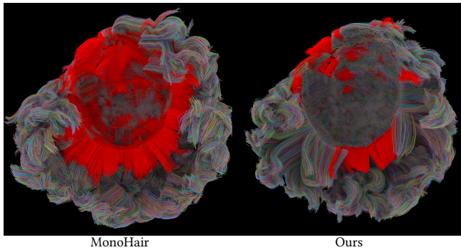
Fig. 14. STRUCTURAL INTEGRITY COMPARISON WITH MONOHAIR. We visualize the inner hair of a curly groom reconstructed using MonoHair [Wu et al. 2024] compared to ours. Short, straight strands, which are undesired, are highlighted in red. Our procedural operators ensure that most strands in a curly groom are curly, whereas MonoHair generates unnatural straight hair.
