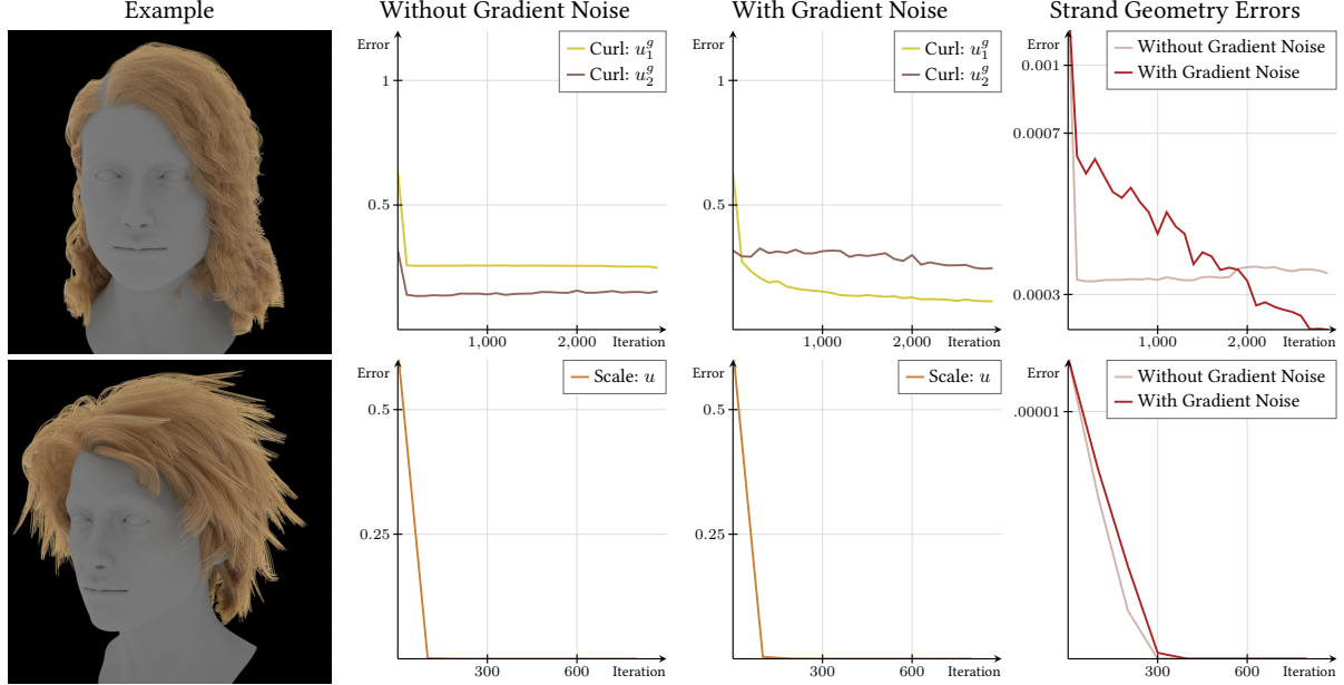
Fig. 17. GRADIENT NOISE. We compare optimizing the operator random numbers with and without adding noise to the gradients. Here, we assume both the guide strands, as well as the operator parameters are known, only the operator random numbers are not known. We measure both the parameter MAE, as well as MSE on the strand vertex positions (shown in log scale). When optimizing for scale, which is a linear function in the random numbers, both methods can optimize to the correct random numbers. When optimizing curl, which is nonlinear in its random numbers, not adding noise quickly gets stuck in a local minima. Adding noise can help escape the local minima and continue reducing the parameter and geometry errors. Groom adapted from Hair Styles ©Daniel Bystedt.
