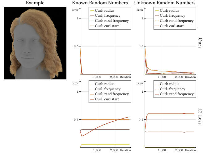
Fig. 15. STRAND SHAPE LOSS. We compare our loss functions in optimizing the curl operator, a strand shape operator, in a synthetic example. Here we assume the guide strands are known, and we compare MAE on the parameter values. When the random numbers are also known, there is a set of parameters that would exactly match the target strands. Even in this case, as curl is a nonlinear function in its parameters, a vertex-wise L2 loss cannot optimize to the correct parameters, whereas ours converges to the exact parameters. When the random numbers are not known, an exact match cannot be expected. Ours converges to within a reasonable tolerance, while the L2 loss still diverges. Groom adapted from Hair Styles ©Daniel Bystedt.
