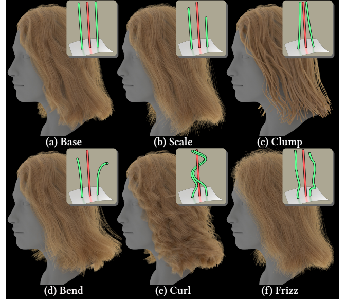
Fig. 3. GROOMING OPERATORS. (a) Given a base hair groom, (b)-(f) shows the effect of each individual operator. For each, a single red operator guide hair is shown in the middle, with two green instanced strands deformed by the operator. The render shows the overall hairstyle change due to each operator. Our pipeline combines operators to produce different grooms. Groom adapted from Hair Styles ©Daniel Bystedt.
