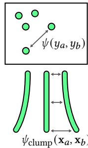
Fig. 6. DPP Loss. DPP theory enables quantifying point clustering through pairwise similarities \psi(y_a, y_b) . To measure hair clumpiness, we define a \psi_{\text{clump}} based on the distance between strands from root to tip.
