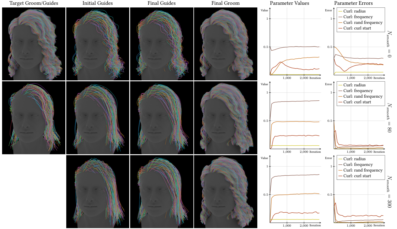
Fig. 11. GUIDE INITIALIZATION SMOOTHING. We analyze the effect of guide smoothing by running our optimization for 3 different amounts of smoothing ( N_{\text{smooth}} = 0, 80, 300 : no smoothing, normal, high). We visualize the initial guides after smoothing, the final guides and groom after the entire optimization pipeline, as well as the parameter values and Mean Absolute Error (MAE) over optimization. When we do not apply any smoothing, the curls are baked into the guides rather than the curl operator. With a high amount of smoothing, the initial guides are nearly straight. Our guide optimization fixes the oversmoothed guides to an extent, but misses some details. Setting N_{\text{smooth}} = 80 recovers the best guides and parameters. Groom adapted from Hair Styles ©Daniel Bystedt.
