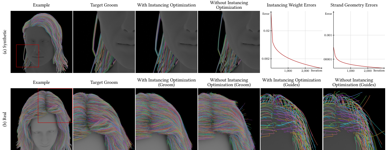
Fig. 12. INSTANCING WEIGHTS OPTIMIZATION. We analyze the effect of optimizing the instancing weights. (a) We construct a synthetic example where all grooming pipeline parameters are known except the instancing weights. Using a simple distance-based interpolation can cause strand differences (note the bundle of hair on the left is too thin). By optimizing for the weights, we can achieve the exact reconstruction, which we validate by comparing Mean Squared Error (MSE) in instancing weights and MSE on strand vertices. (b) On real examples, optimizing the instancing weights can prevent issues during guide optimization when dense strands are poorly interpolated using a distance-based interpolation. Synthetic groom adapted from Hair Styles ©Daniel Bystedt.
