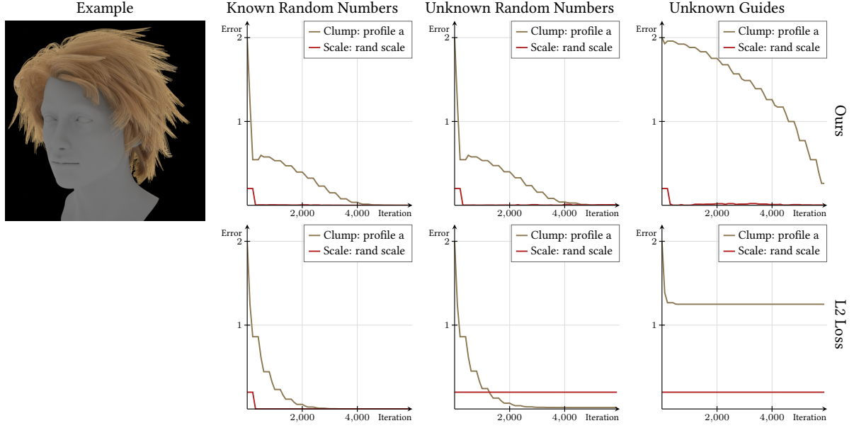
Fig. 16. STRAND CORRELATION LOSS. We compare our loss functions in optimizing the clump and scale operators, which are strand correlation operators, in a synthetic example. We compare MAE on the parameter values. First, we assume the guide strands are known. When the random numbers are also known, there is a set of parameters that would exactly match the target strands. As both operators are monotonic functions in their parameters, both our loss and the vertex-wise L2 loss can optimize to the correct parameters. When the random numbers are not known, an exact match cannot be expected. Both our loss and the L2 loss can optimize the clump operator, which has no random parameters, but only our loss can optimize the scale operator. When neither the guides nor the random numbers are known, our loss can optimize to parameters within a reasonable tolerance, while the L2 loss can optimize neither. Groom adapted from Hair Styles ©Daniel Bystedt.
