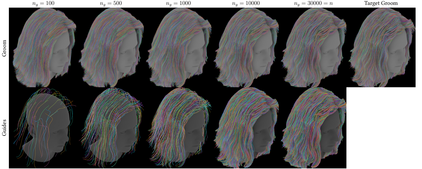
Fig. 18. NUMBER OF GUIDES. We compare the effect of the number of guide strands on the optimization, from n_g = 100 , to n_g = 30000 , which is the same number of guides as the number of dense strands n . As we increase the number of guides, we can match more detail in the target groom. However, increasing the number of guides reduces the ease of editing the procedural groom.
