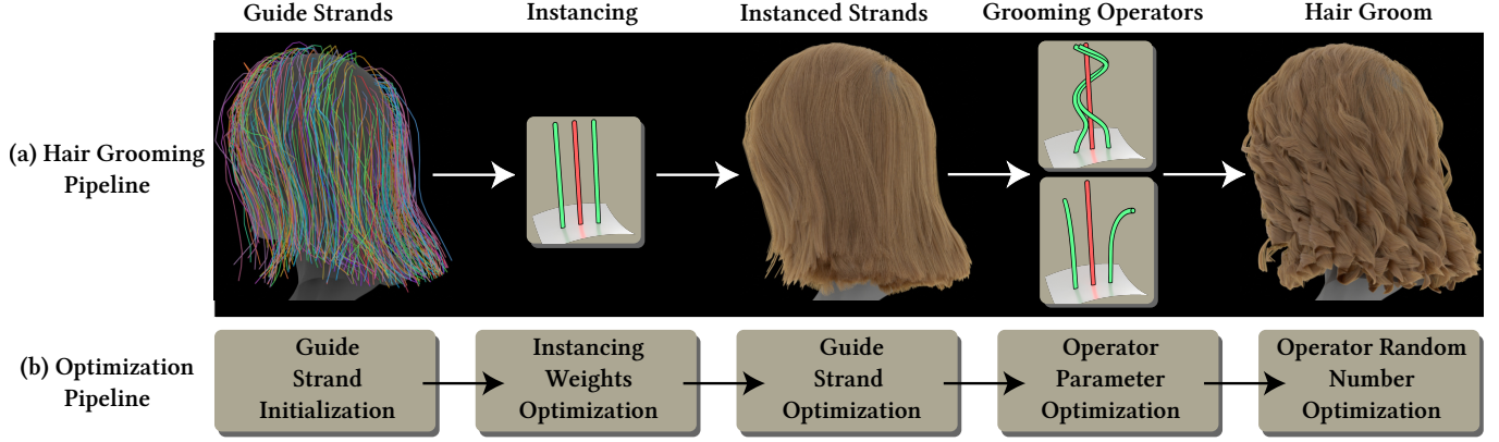
Fig. 2. PIPELINES. (a) Our hair grooming pipeline takes a sparse set of guide strands, instances them to dense strands, and then procedurally deforms them using grooming operators to generate the hair groom. (b) To optimize the various parameters in the hair grooming pipeline, we initialize the guide strands using the target strands. We optimize the weights of the instancing operation and the shape of the guide strands. We then optimize both the operator parameters, which control the global hairstyle, as well as operator random numbers, to refine individual strands. Groom adapted from Hair Styles ©Daniel Bystedt.
