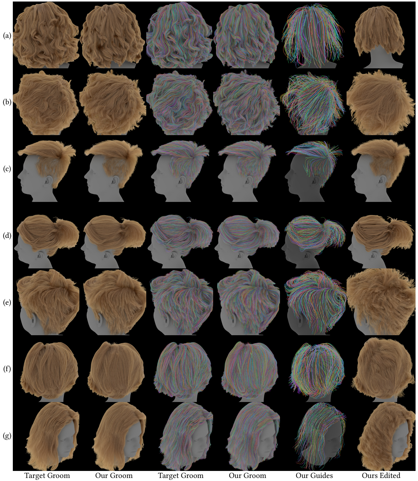
Fig. 8. REAL GROOMS. We recover the guide strands and operator parameters of 7 grooms from previous reconstruction work. We visualize the non-procedural target grooms and our recovered grooms and guides. We also show a simple procedural edit for each.
