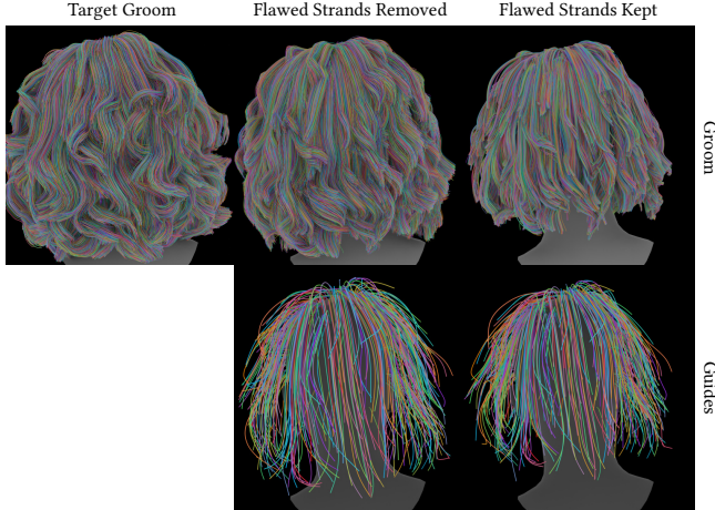
Fig. 13. REMOVING FLAWED STRANDS. Neural hair reconstruction methods that infer inner hair using data-driven priors can have flawed strands. For example, in this groom, the inner hair in the back is short and straight, rather than curly as expected, as seen in Figure 14. Optimizing using these flawed strands causes the guide optimization to fit to the short strands, reducing the hair length of the back. Removing the flawed strands helps prevent this.
