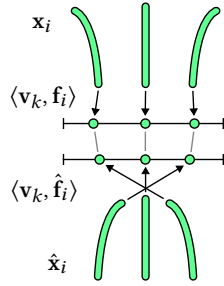
Fig. 5. SLICED WASSERSTEIN LOSS. To compare two sets of hair strands ( \mathbf{x}_i, \hat{\mathbf{x}}_i ) without known strand correspondences, each strand's features ( \mathbf{f}_i, \hat{\mathbf{f}}_i ) are projected to scalars ( \langle \mathbf{v}_k, \mathbf{f}_i \rangle, \langle \mathbf{v}_k, \hat{\mathbf{f}}_i \rangle ). Both sets are sorted and compared using an L2 loss.
