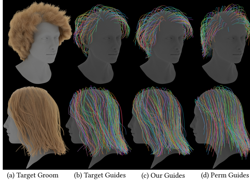
Fig. 20. COMPARISON WITH PERM. Given target grooms (a), our guide clustering and optimization (c) result in more accurate guide strands (b) compared to the learned guide strand generation of Perm [He et al. 2024] (d). Grooms adapted from Hair Styles ©Daniel Bystedt.
