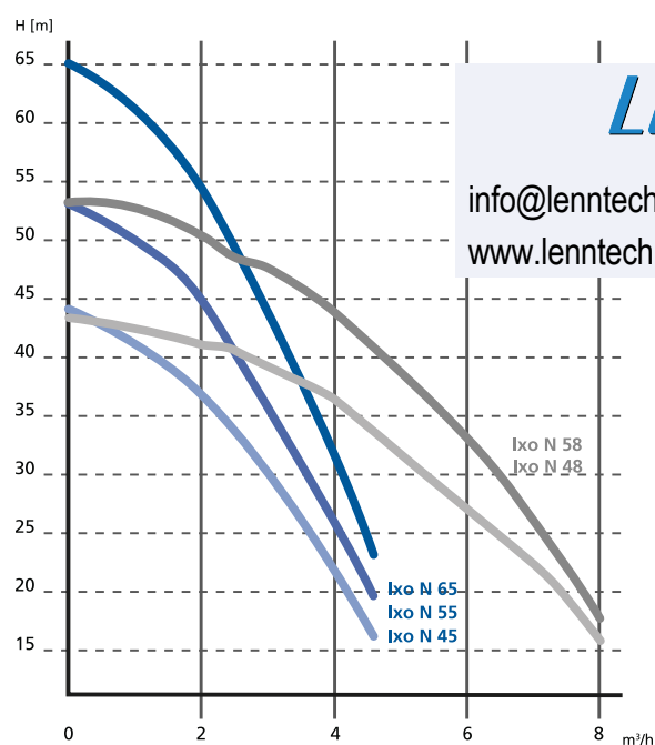
Ixo N characteristic curves
