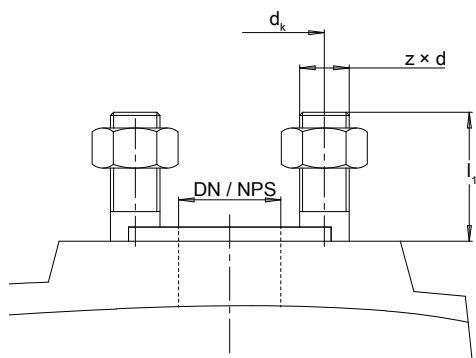
Fig. 5: Flange dimensions
