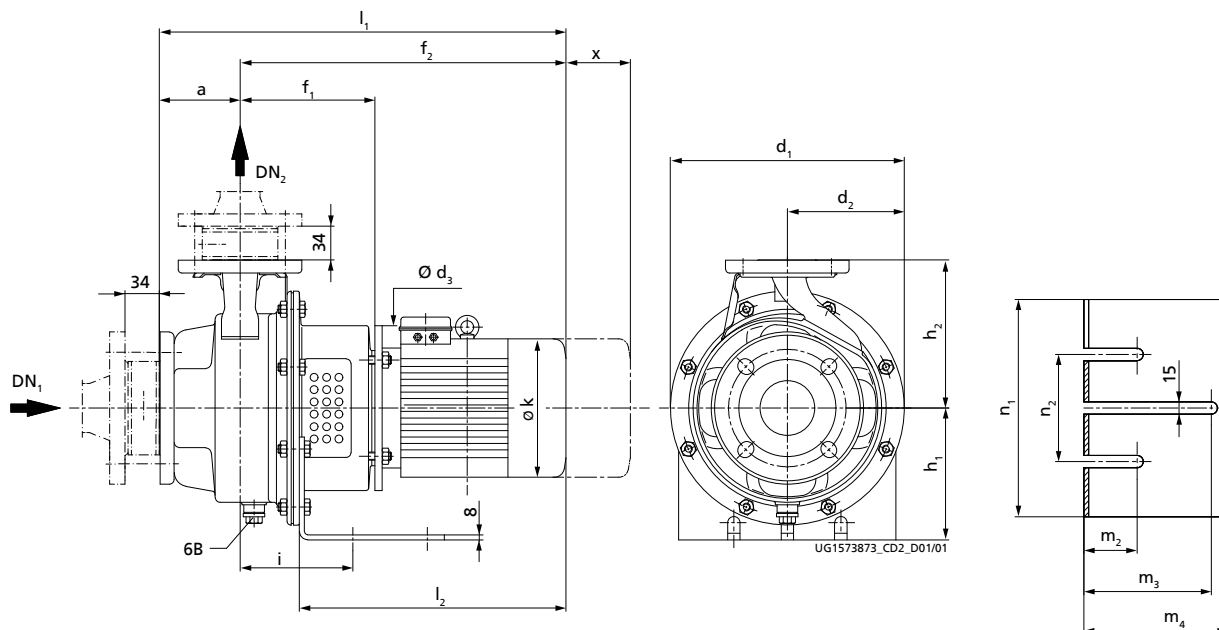
Fig. 9: Etachrom B with pump foot, dimensions [mm]
