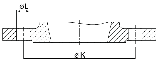
Fig. 17: Flange (example)
