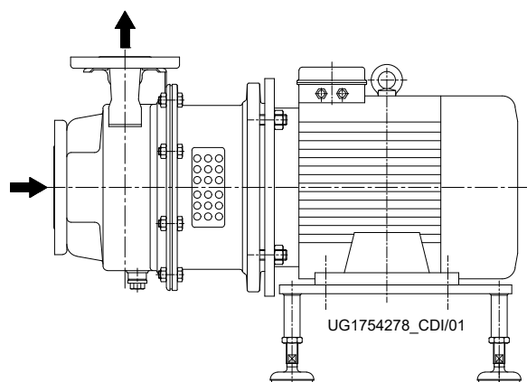
Fig. 22: Machine mount, motor sizes 80 = 0.55 kW to 225 = 45 kW
