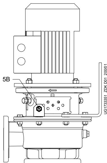
Fig. 24: Illustration of closing element with vent function
