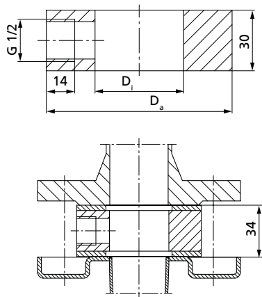
Fig. 16: Dimensions of the pressure gauge connection (intermediate flange) [mm]
