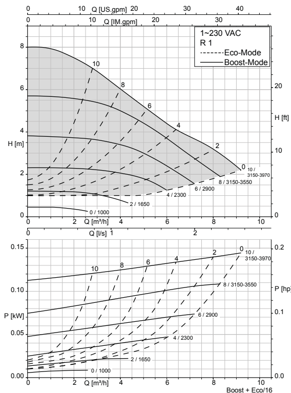
Calio 25-80 Boost, Eco Mode
