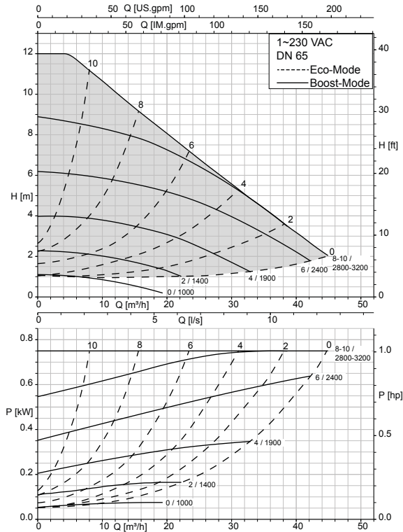
Calio 65-120 Boost, Eco Mode
