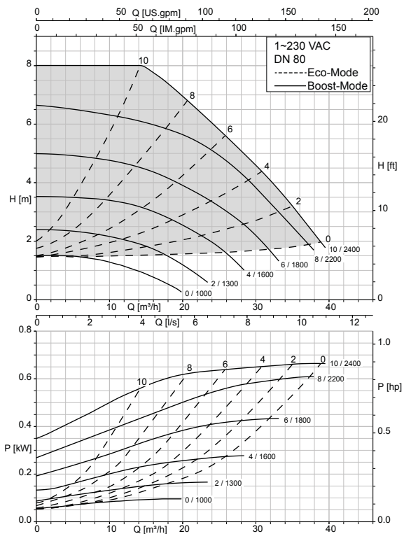
Calio 80-80 Boost, Eco Mode
