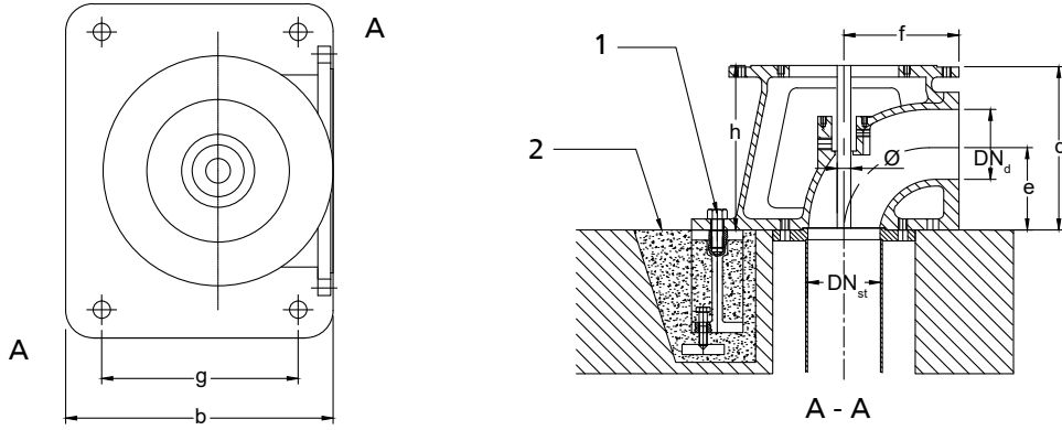
Fig. 1: Discharge nozzle dimensions VN 1342, 1342A, 1830 and 2030
