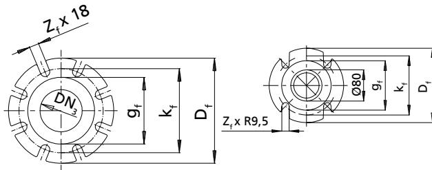
Dimensions of flanged bend DN 3 [mm]
